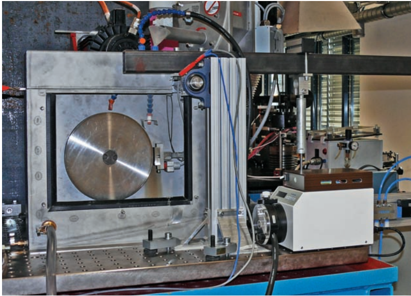
2 Block-on-ring test bench for testing slide friction wear and three-body abrasion.
