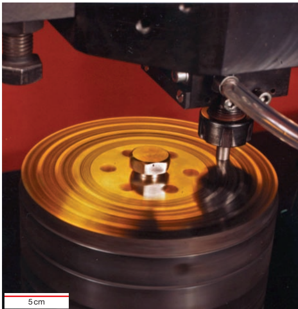
8 Pin-disk arrangement for the determination of sliding and static friction coefficients. Operation is possible both with lubricant and under a defined atmosphere.
