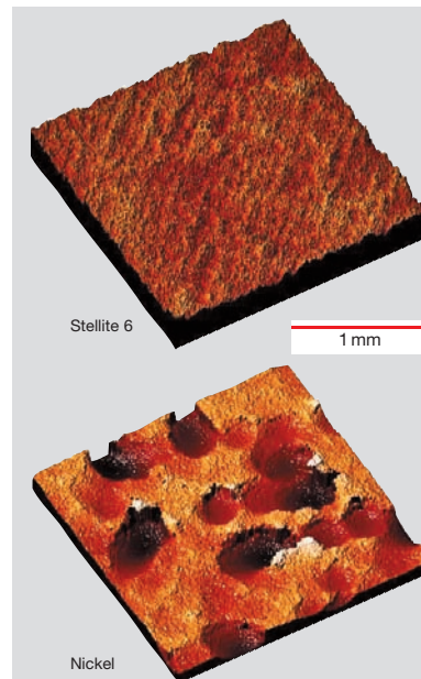
6 Clear differences can be seen in the surface structures of Stellite 6 and nickel after the cavitation test.
