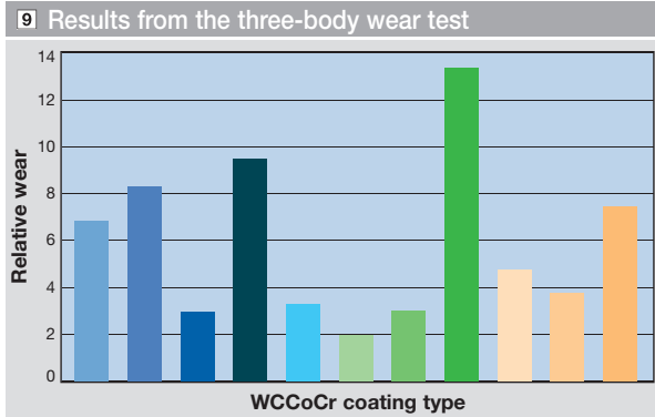
Differences in the three-body wear of thermally sprayed protective coatings of the same metallurgical composition.
