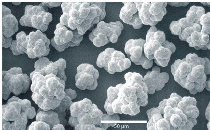
SEM micrograph showing typical size, shape and surface morphology of SF Nickel Powder
