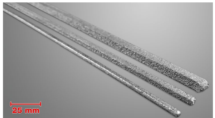
Top: SEM photomicrographs of Metco 51151B, showing morphology that is typical for these products. Bottom: Metco 81586 welding rods.
