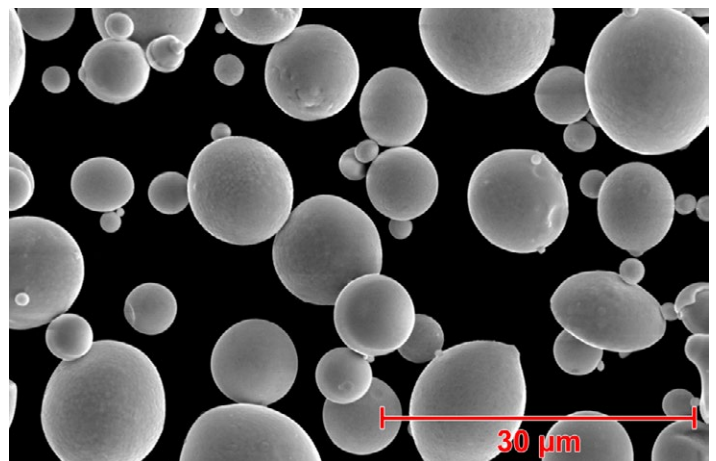
SEM photomicrograph showing the typical gas atomized morphology of a proprietary Oerlikon Metco MCrAlY material
