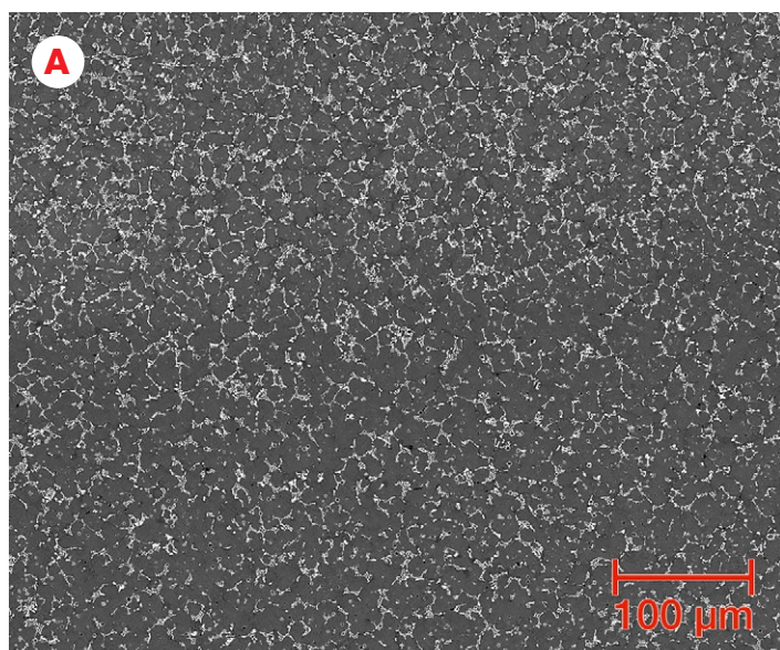
Microstructure comparison of Metco 8248 GMAW deposit [A] versus WC-Ni GMAW deposit [B]. Note the carbide spacing is thermodynamically driven to a very precise spacing and fine hard phase size in the Metco 8248 GMAW deposit versus the very large hard phase particles in the WC-Ni GMAW deposit.
