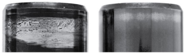
Positive effects of BALINIT® DLC coated wrist pins. 经BALINIT® DLC涂层的活塞销效果
