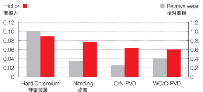
Positive effects of BALINIT® DLC coated wrist pins. 经BALINIT® DLC涂层的活塞销效果
