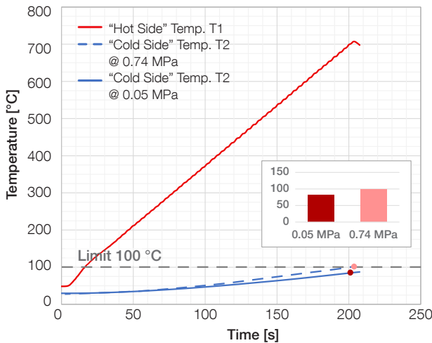
Thermal Characterization @ 0.05 MPa
