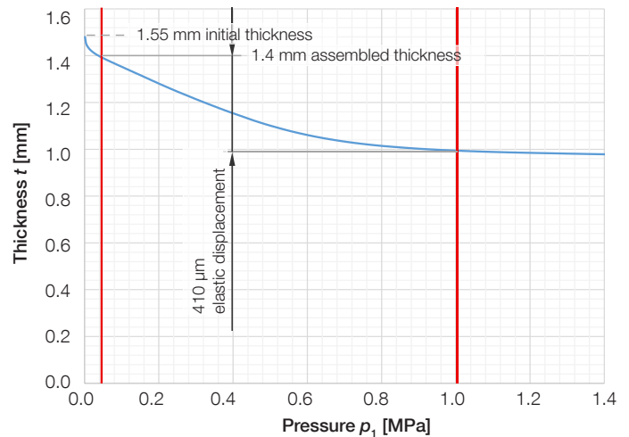
Mechanical Characterization
