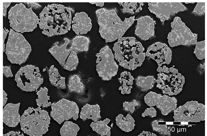
SEM Photomicrographs showing the morphology (top) and the microstructure (bottom) of Woka 7507.
