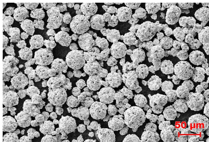
SEM of Metco 5280A show typical morphology of these powders
