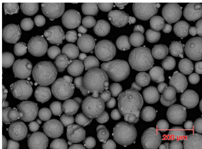
SEM photomicrograph of Metco 1720A showing morphology that is typical of these products.
