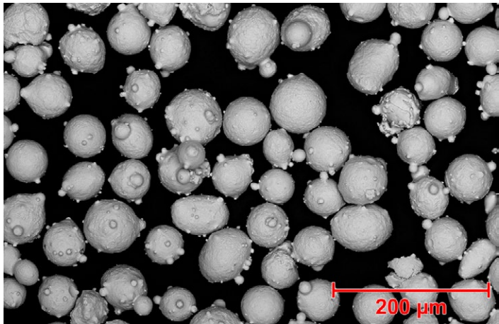
SEM photomicrograph of Amdry 995C, showing the gas atomized morphology typical of these materials.
