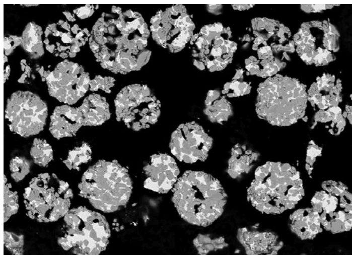
SEM photomicrographs showing the morphology (top) and the microstructure (bottom) of a Woka 7200 series materials.
