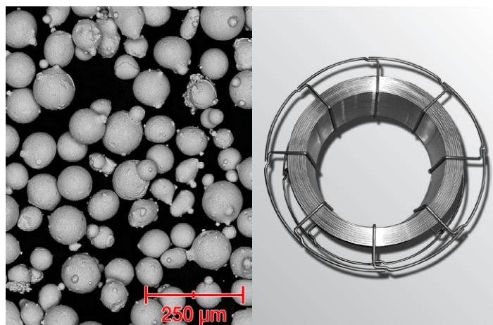
Left: Gas-atomized Metco 1221A showing typical morphology of powder products. Right: Packaging for composite wire products.
