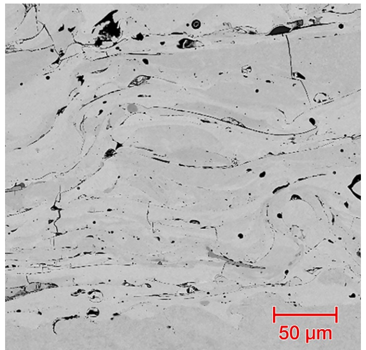
Typical as-sprayed coating microstructure of Metco 8201.
