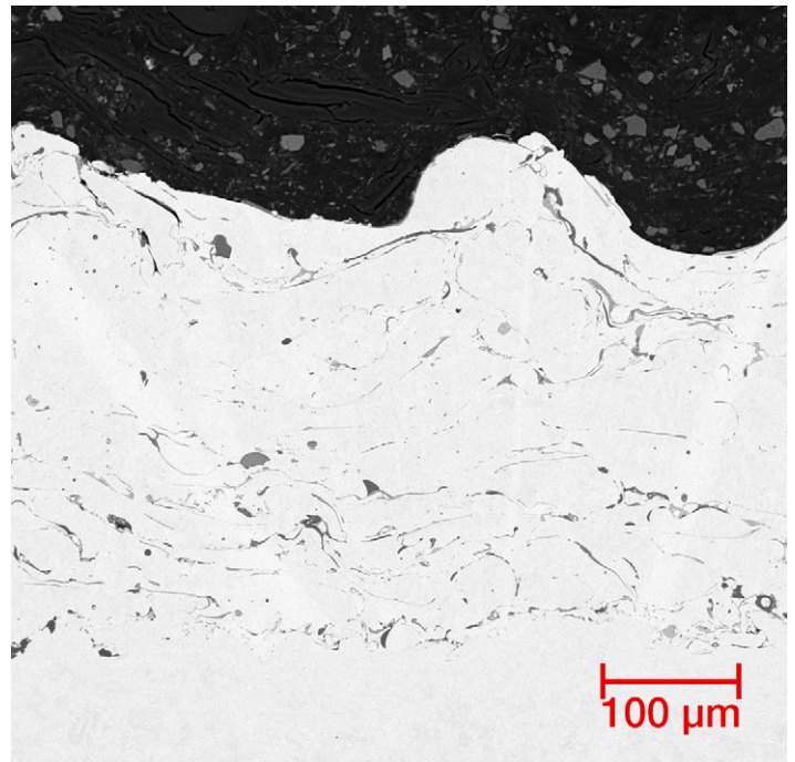
Typical as-sprayed coating microstructure of Metco 8293.
