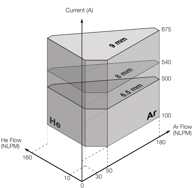
Argon/Helium Operation - 6.5 mm, 8 mm and 9 mm Nozzle
