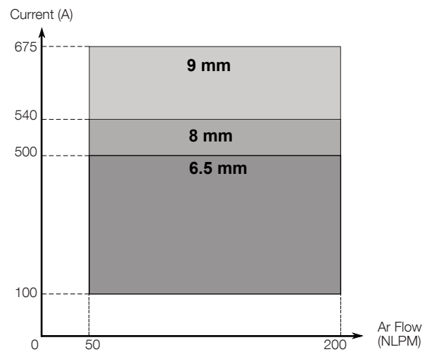
Argon Operation - 6.5 mm, 8 mm and 9 mm Nozzle
