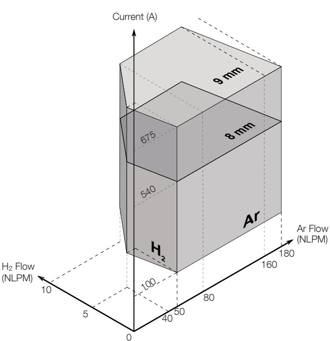
Argon/Hydrogen Operation – 8 mm and 9 mm Nozzle
