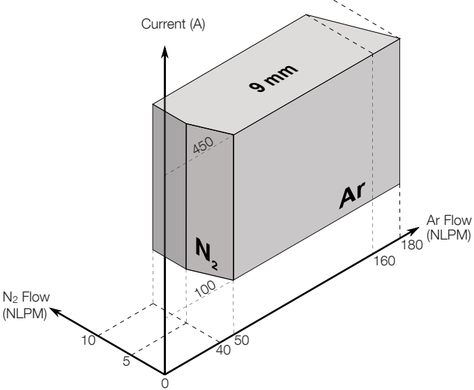
Argon/Nitrogen Operation - 9 mm Nozzle
